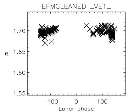
EFMCLEANED _VE1_ Non-UNI. skypatch removed_VE1_ Non-UNI. skypatch removed
