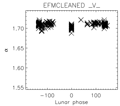
EFMCLEANED _V_ Non-UNI. skypatch removed_V_ Non-UNI. skypatch removed
