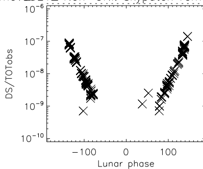
EFMCLEANED _VE2_ Non-UNI. skypatch removed_VE2_ Non-UNI. skypatch removed
