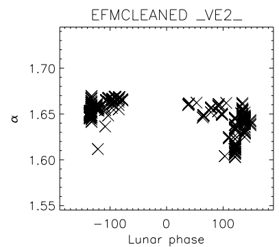
EFMCLEANED _VE2_ Non-UNI. skypatch removed_VE2_ Non-UNI. skypatch removed
