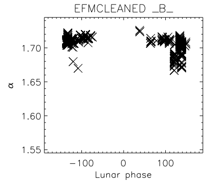
EFMCLEANED _B_ Non-UNI. skypatch removed_B_ Non-UNI. skypatch removed
