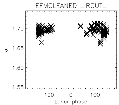
EFMCLEANED _JRCUT_ Non-UNI. skypatch removed_JRCUT_ Non-UNI. skypatch removed
