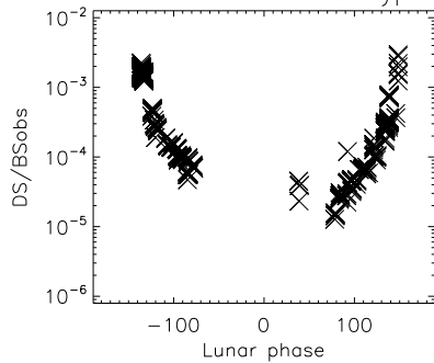
EFMCLEANED _JRCUT_ Non-UNI. skypatch removed_JRCUT_ Non-UNI. skypatch removed
