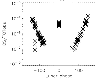
EFMCLEANED _VE1_ Non-UNI. skypatch removed_VE1_ Non-UNI. skypatch removed
