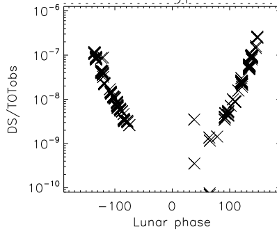
EFMCLEANED _V_ Non-UNI. skypatch removed_V_ Non-UNI. skypatch removed
